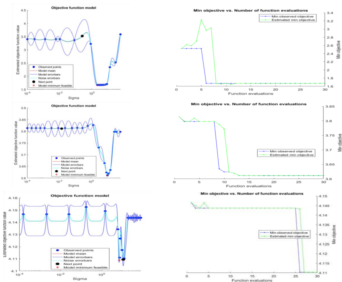
Picture3: finding sigma parameter in GPR algorithm by bayes algorithm of the current year first line, next year second line, next two year third line in the first Fold
