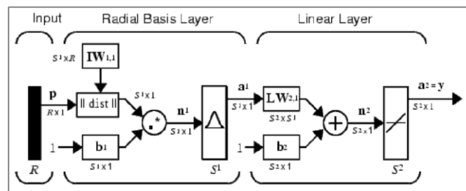
Picture 2: a general model of a RBF network with R input data
